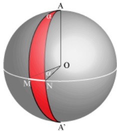
The area of a spherical wedge
