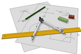
Geometry by construction, not calculation
