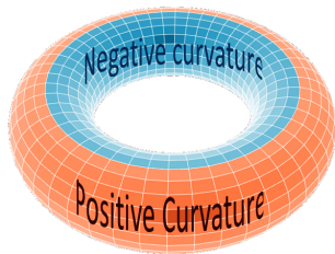
Curvature zones of a torus
