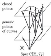
The primes as a geometric space
