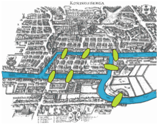
Geometry without distance
