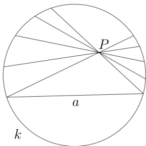
Hyperbolic lines as Euclidean chords
