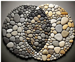
Open sets are almost everywhere
