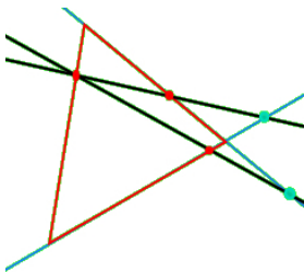
A line entering a triangle must exit it
