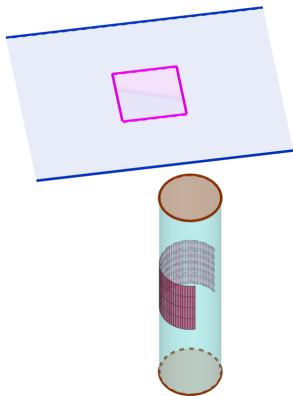
Bending without stretching
