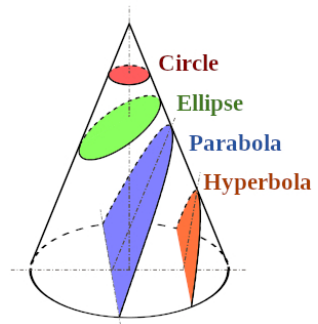
One curve, different infinite boundaries
