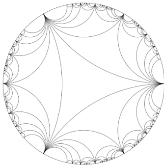
Poincaré's conformal model
