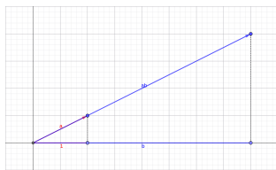
Descartes' multiplication: ab is a line
