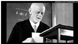
Hilbert's 23 problems for the 20 th century
