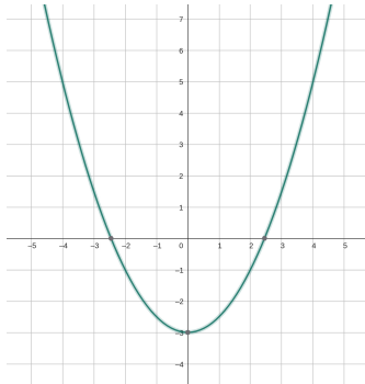
Illustrating the Cartesian coordinate system
