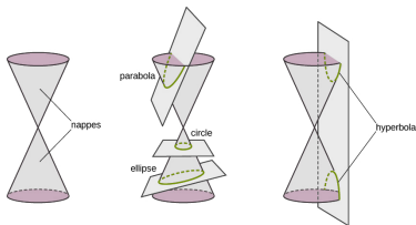
Conic sections from a double-napped cone
