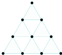
The Tetractys
