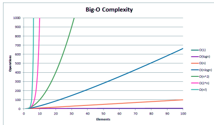
Polynomial vs. exponential time growth
