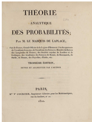
Laplace's seminal work on probability
