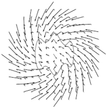
Brouwer's fixed-point theorem in 2D
