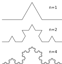
Koch curve
