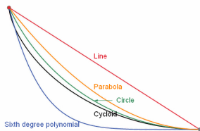
The brachistochrone problem solution (a cycloid)
