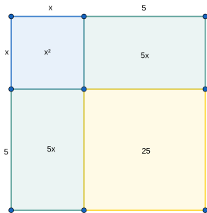
Al-Khwarizmi's geometric method for x^2 + 10x = 39
