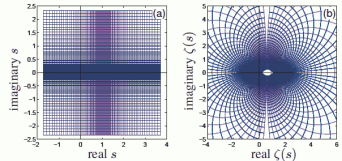
The critical line for the Riemann zeta function
