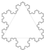
Koch snowflake
