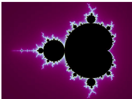
The Mandelbrot set
