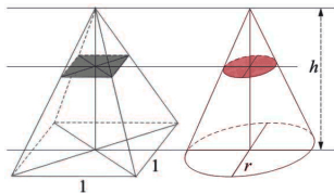
Cavalieri's principle for volumes
