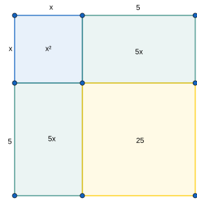
Al-Khwarizmi's geometric method for x^2 + 10x = 39
