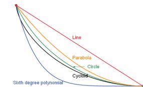
The brachistochrone problem solution (a cycloid)
