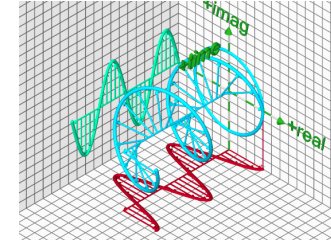
Visualising Euler's formula on the complex plane
