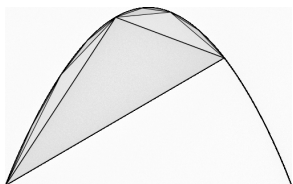
Quadrature of the parabola
