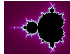
The Mandelbrot set
