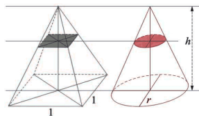
Cavalieri's principle for volumes
