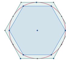
Inscribed and circumscribed polygons
