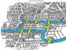
The Königsberg bridge problem
