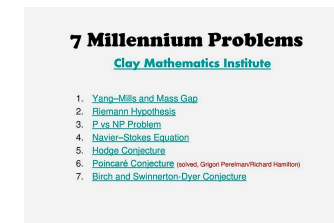
The Clay Millennium Prize problems
