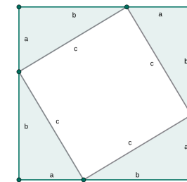
Rearrangement proof of a^2 + b^2 = c^2
