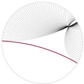
Visualising hyperbolic geometry: Poincaré disk model
