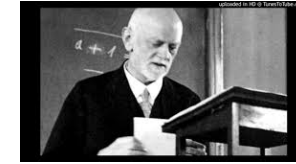
Hilbert's 23 problems for the 20 th century
