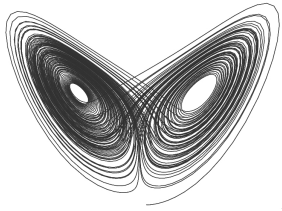
The Lorenz attractor
