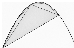
Quadrature of the parabola
